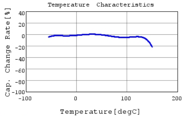
RHEL81H471K0A2H03B C-Temp. capchange, DCOV,
