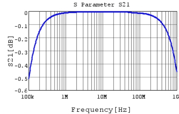
RHEL82A473K1K1H03B S21 DCOV, 25degC
