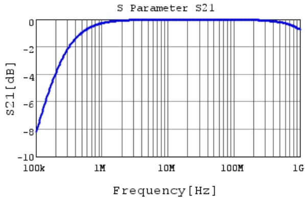
RHEL82A682K0M1H03A S21 DCOV, 25degC
