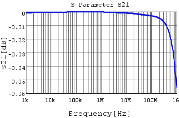
ECASD60E477M006K00 S21 DCOV, 25degC
