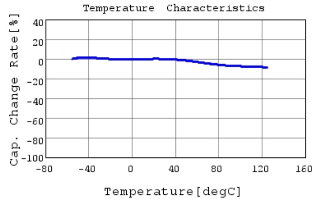
GCJ188R72A472KA01 C-Temp. capchange, DC0.0V,
