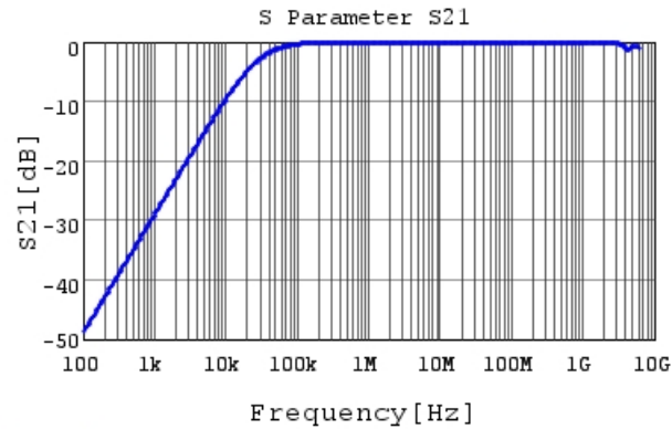
GCJ21BR71H563KA01 S21 DC0V, 25degC
