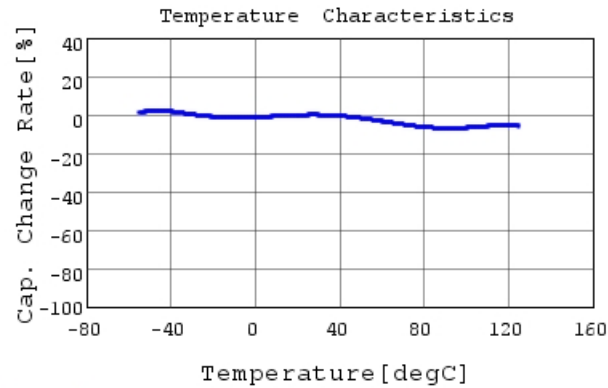
GCJ21BR71H563KA01 C-Temp. capchange, DC0.0V,
