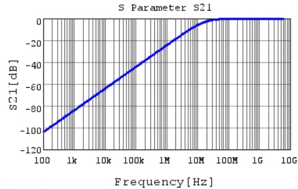
GCM033R71E101KA03 S21 DC0V,25degC
