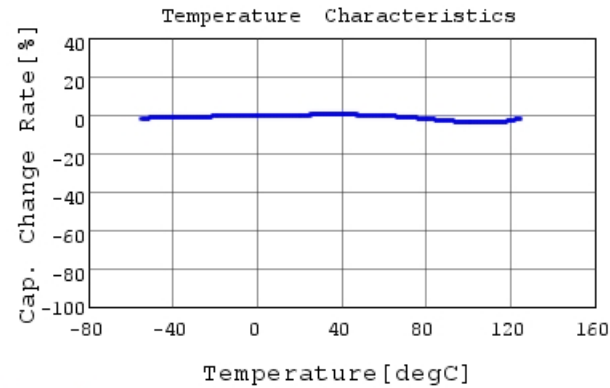
GCM033R71E101KA03 C-Temp. capchange, DC0.0V,
