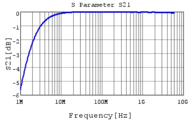
GCM1555G1H102FA16 S21 DC0V, 25degC
