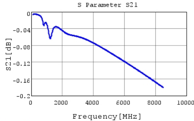
GCM1555G1H561GA16 S21 DC0V, 25degC
