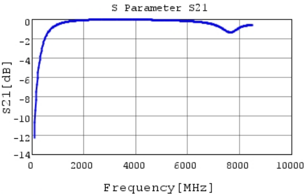
GCM1885C2A4R0CA16 S21 DCOV, 25degC
