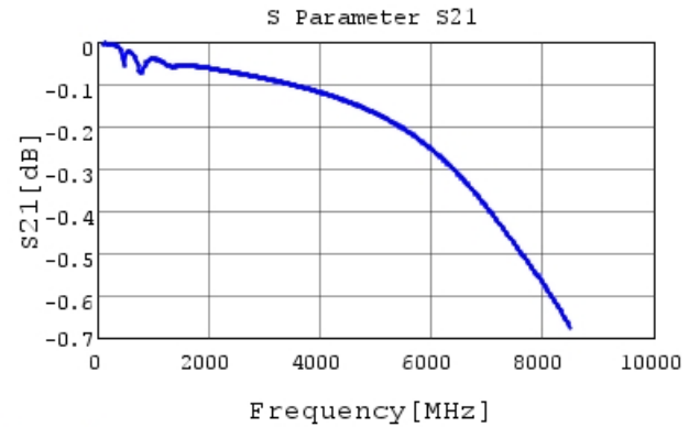
GCM1885C2A821JA16 S21 DCOV, 25degC
