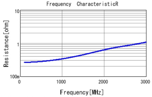
GCM21A5C2E330JX01 R DC0V, 25degC
