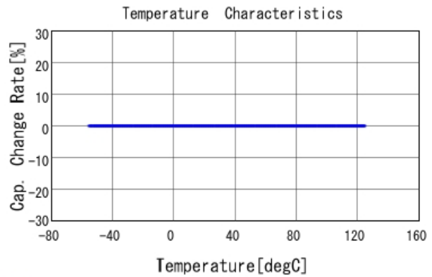
GCM21A5C2E330JX01 C-Temp. capchange, DC0V, AC1Vrms
