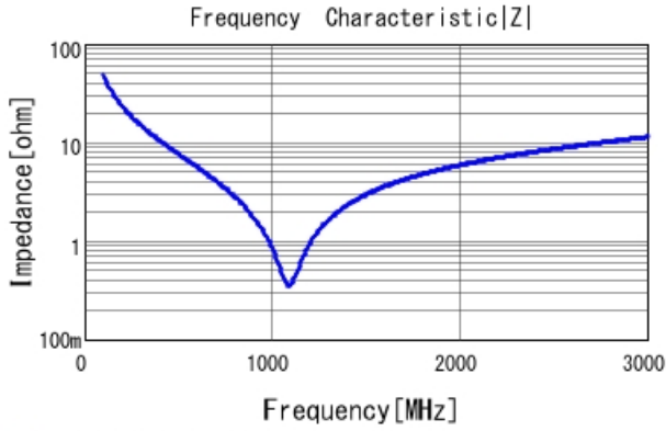
GCM21A5C2E330JX01 |Z| DC0V, 25degC
