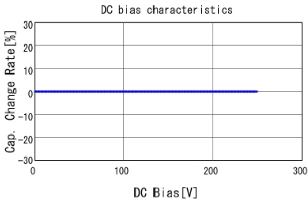
GCM21A5C2E330JX01 C-DC bias capchange, 25.0degC, AC1V
