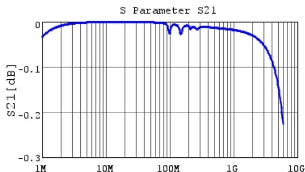
Frequency [Hz] GCM21B5C1K183JA16 S21 DCOV, 25degC
