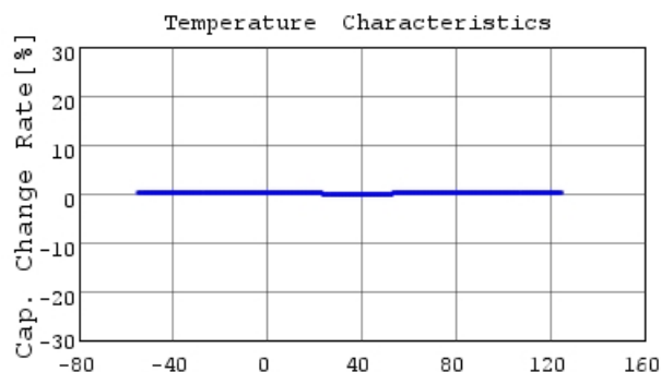
Temperature [degC] GCM21B5C1K183JA16 C-Temp. capchange, DCOV, 1
