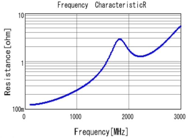
GCM31A7U3A680JX01 R DC0V, 25degC
