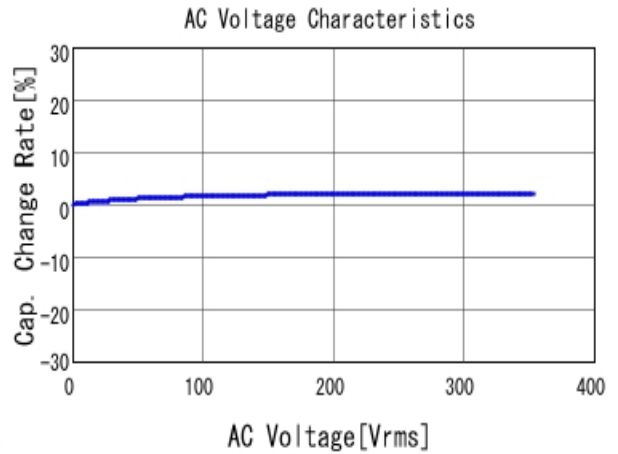
GCM31A7U3A680JX01 C-AC Voltage capchange, DC0V, 25.0d
