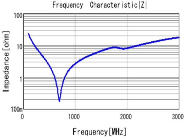
GCM31A7U3A680JX01 |Z| DC0V, 25degC
