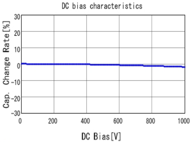
GCM31A7U3A680JX01 C-DC bias capchange, 25.0degC, AC1V
