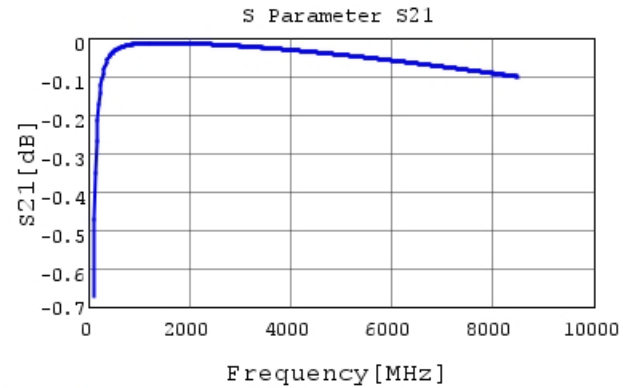
GRM0115C1E390GE01 S21 DCOV, 25degC
