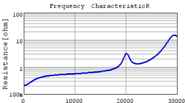
GRM0223C1H2R6CA03 R DCOV, 20degC
