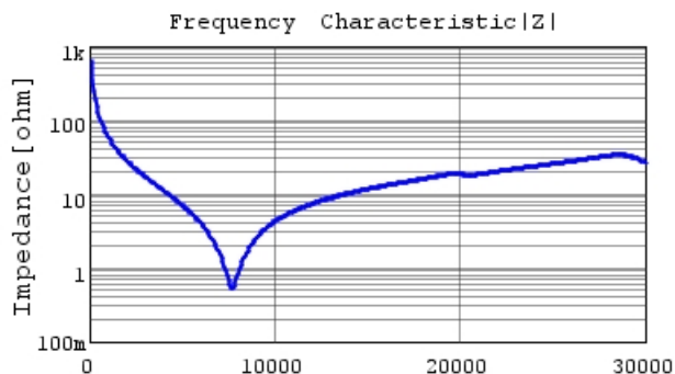
GRM0223C1H2R6CA03 |Z| DCOV, 20degC
