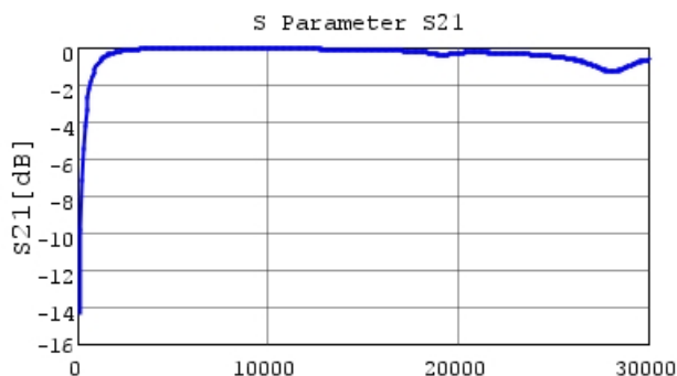
GRM0223C1H3R1CA03 S21 DCOV, 20degC
