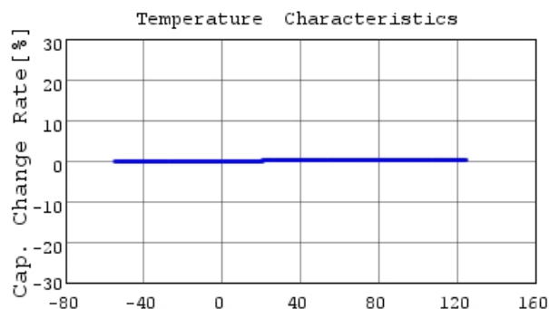
GRM0223C1H3R1CA03 C-Temp. capchange, DCOV, 1
