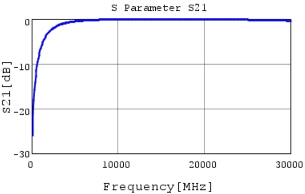
GRM0224C1HR80WA03 S21 DCOV, 20degC
