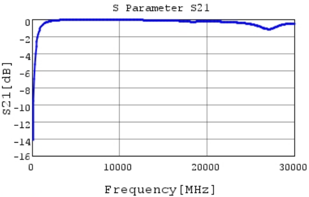
GRM0225C1H3R2WA03 S21 DCOV, 25degC
