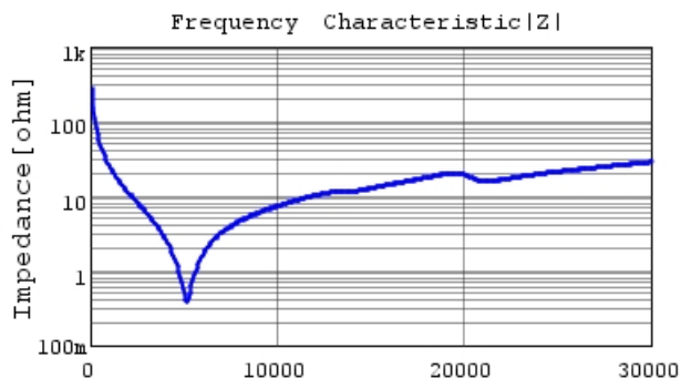
GRM0225C1H5R9BA03 |Z| DCOV,25degC
