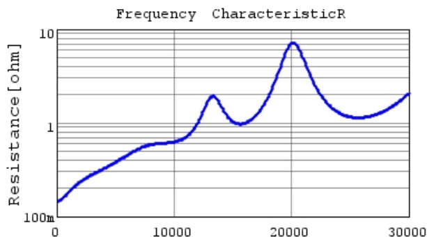
GRM0225C1H5R9BA03 R DCOV,25degC
