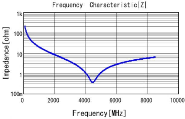
■ GRM0225C1H7R6WA03 |Z| DCOV, 25degC
