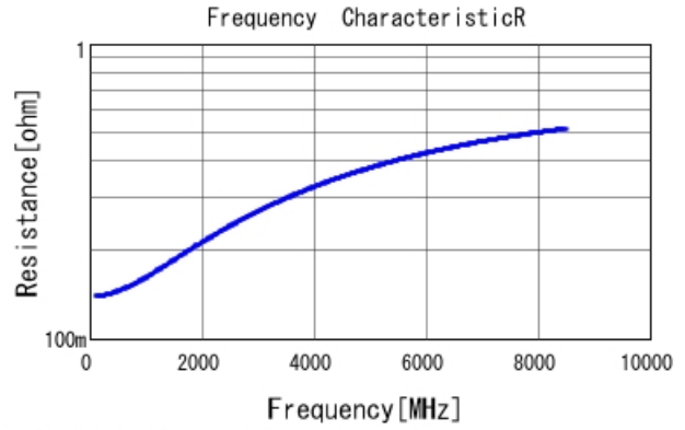
■ GRM0225C1H7R6WA03 R DCOV, 25degC
