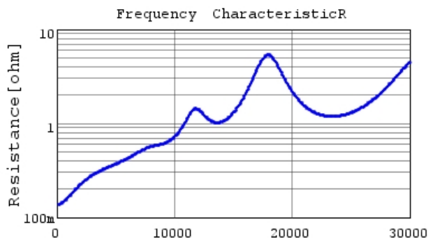
GRM0225C1H7R9CA03 R DCOV,25degC
