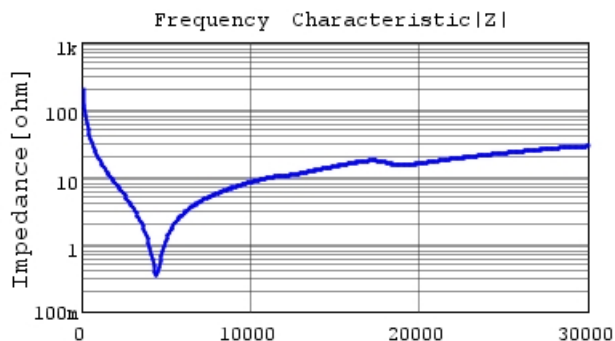
GRM0225C1H7R9CA03 |Z| DCOV,25degC
