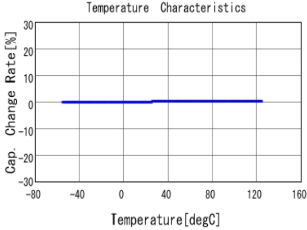
■ GRM0225C1H8R0DA03 C-Temp. capchange, DCOV, AC1Vrms
