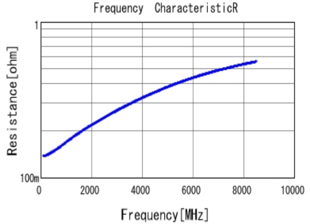
■ GRM0225C1H8R0DA03 R DCOV, 25degC
