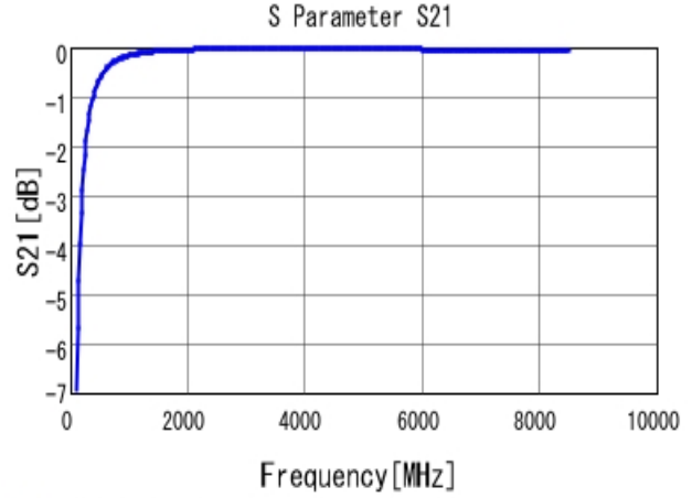
■ GRM0225C1H8R0DA03 S21 DCOV, 25degC
