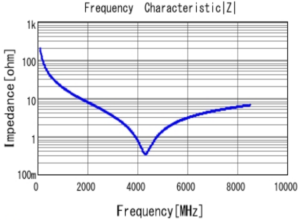
■ GRM0225C1H8R0DA03 |Z| DCOV, 25degC
