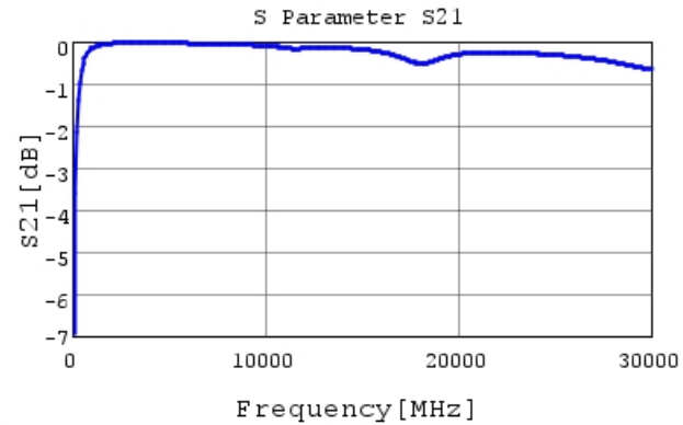
GRM0225C1H8R0WA03 S21 DCOV, 25degC
