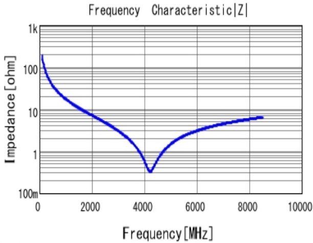
■ GRM0225C1H8R6DA03 |Z| DCOV, 25degC
