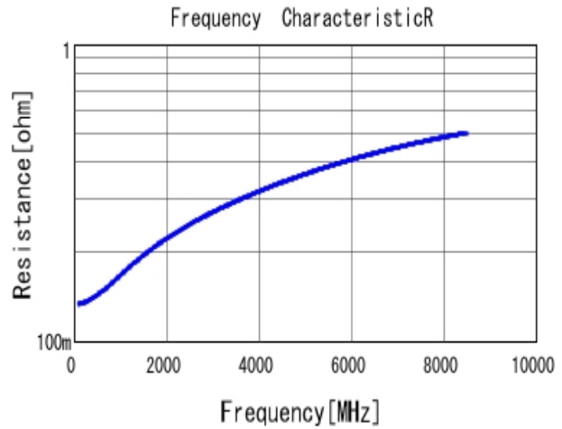
■ GRM0225C1H8R6DA03 R DCOV, 25degC
