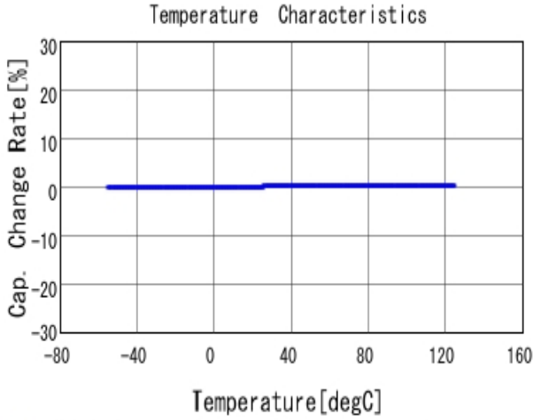
■ GRM0225C1H8R6DA03 C-Temp. capchange, DCOV, AC1Vrms
