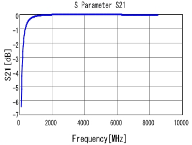
■ GRM0225C1H8R6DA03 S21 DCOV, 25degC
