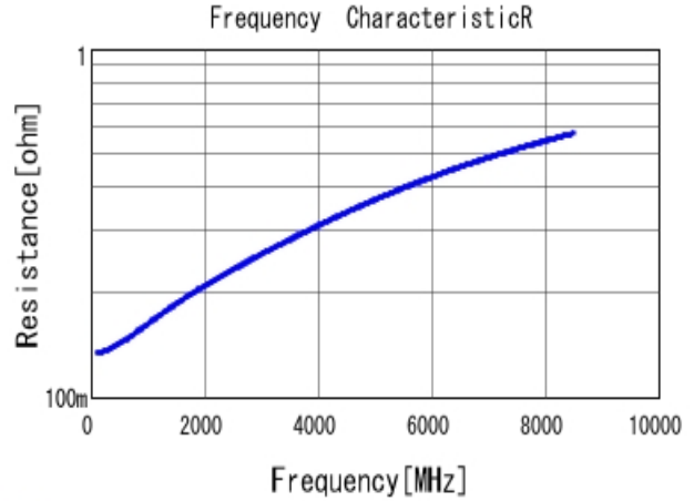
■ GRM0225C1H9R1CA03 R DCOV, 25degC
