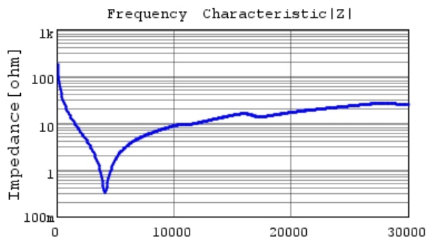
GRM0225C1H9R1CA03 |Z| DCOV,25degC
