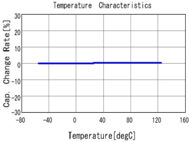
■ GRM0225C1H9R1CA03 C-Temp. capchange, DCOV, AC1Vrms
