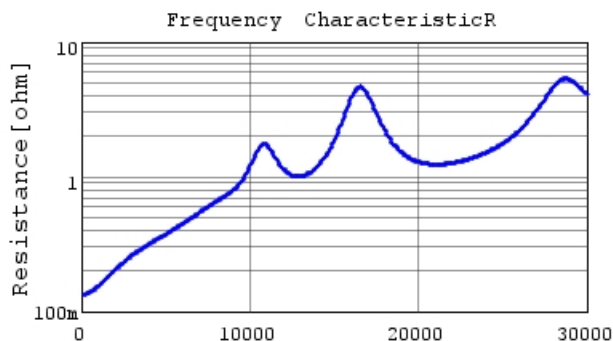
GRM0225C1H9R1CA03 R DCOV,25degC
