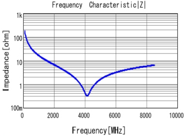
■ GRM0225C1H9R1CA03 |Z| DCOV, 25degC
