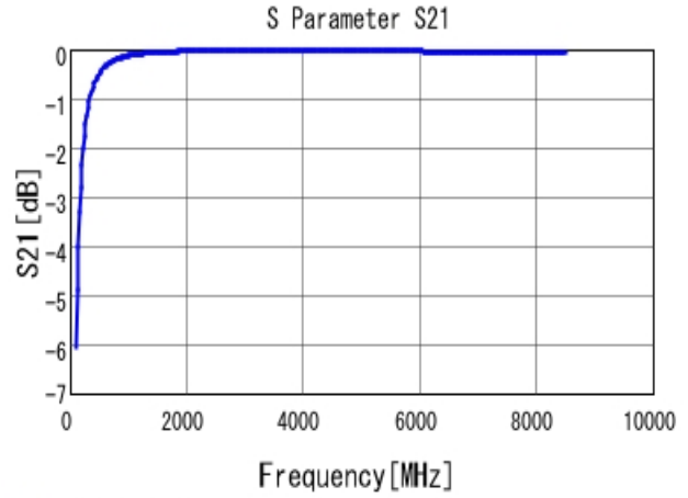
■ GRM0225C1H9R1CA03 S21 DCOV, 25degC
