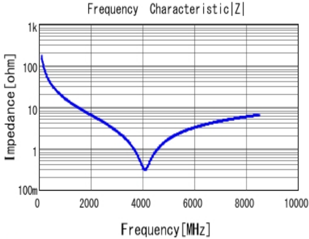
■ GRM0225C1H9R4DA03 |Z| DCOV, 25degC
