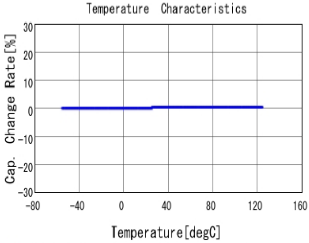
■ GRM0225C1H9R4DA03 C-Temp. capchange, DCOV, AC1Vrms
