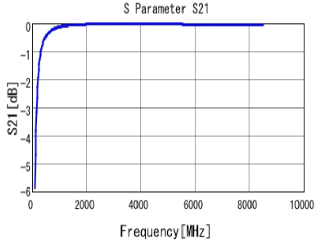
■ GRM0225C1H9R4DA03 S21 DCOV, 25degC
