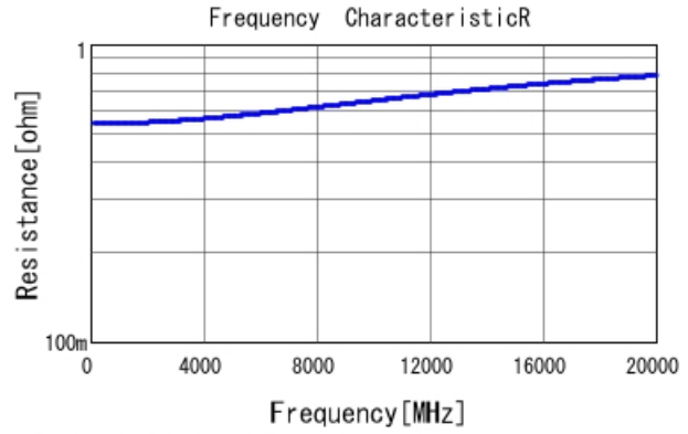
■ GRM0225C1HR80BA03 R DCOV, 25degC
