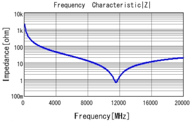
■ GRM0225C1HR80BA03 |Z| DCOV, 25degC
