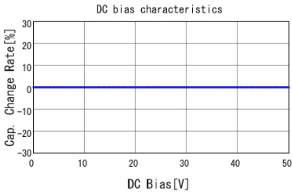
■ GRM0225C1HR80BA03 C-DC bias capchange, 25.0degC, AC1V
