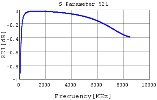
GRM0332C2A330JA01 S21 DCOV, 20degC
