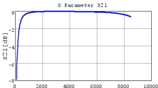
GRM0332C2A7R0DA01 S21 DCOV, 20degC
