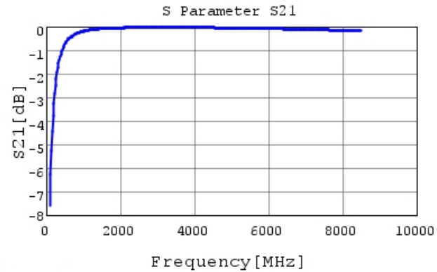
GRM0332C2A7R3BA01 S21 DCOV, 20degC
