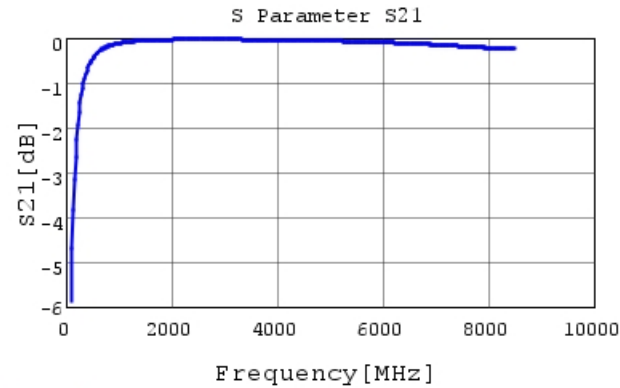
GRM0332C2A9R4CA01 S21 DCOV, 20degC
