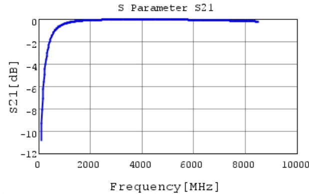
GRM0335C1H4R8CA01 S21 DCOV, 25degC
