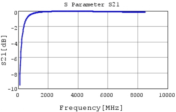
GRM0335C1H5R6DA01 S21 DCOV, 25degC
