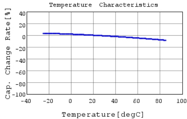
GRM033B11A103KA01 C-Temp. capchange, DC0.0V,
