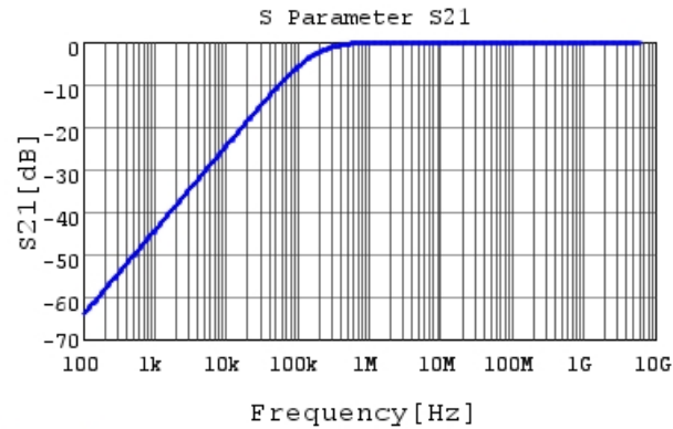
GRM033B11A103KA01 S21 DC0V,20degC
