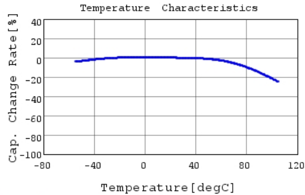
GRM033D80E225ME47 C-Temp. capchange, DC0.0V,
