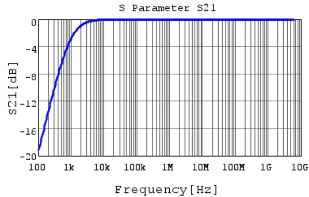
GRM033D80E225ME47 S21 DC0V, 25degC
