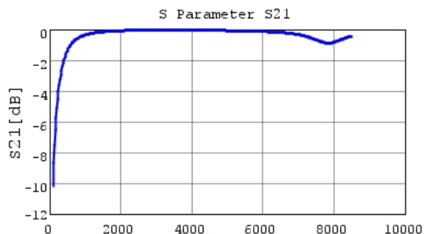
GRM1552C2A5R2DA01 S21 DCOV, 20degC
