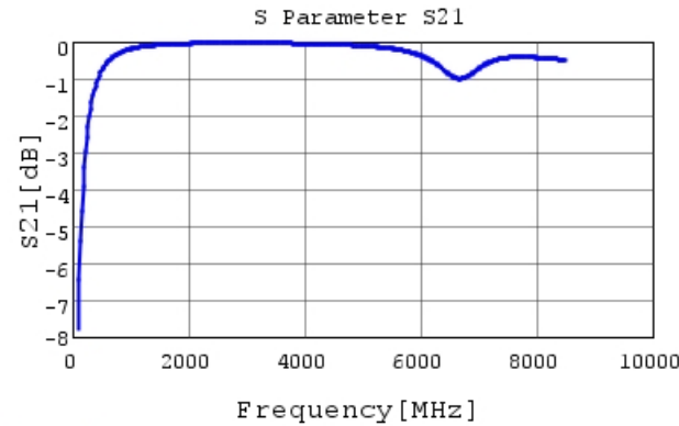
GRM1552C2A7R1CA01 S21 DC0V, 20degC
