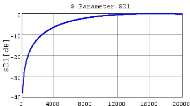
GRM1554C2AR20WA01 S21 DCOV, 20degC
