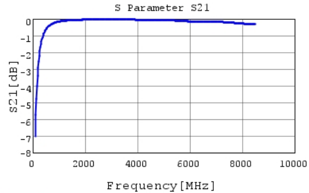
GRM1555C2A7R9DA01 S21 DC0V, 25degC
