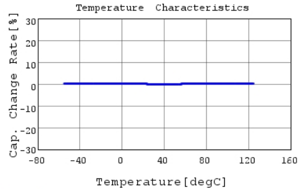
GRM1555C2A7R9DA01 C-Temp. capchange, DC0V, 1
