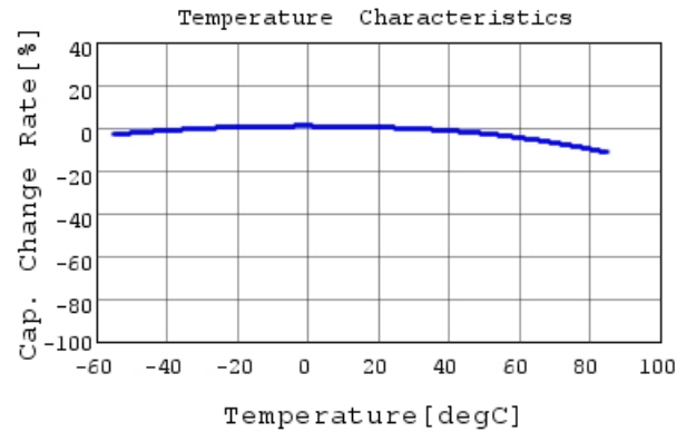
GRM155R60J474KE19 C-Temp. capchange, DC0.0V,
