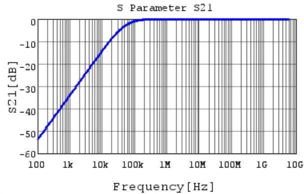
GRM155R61C333KA01 S21 DC0V, 25degC
