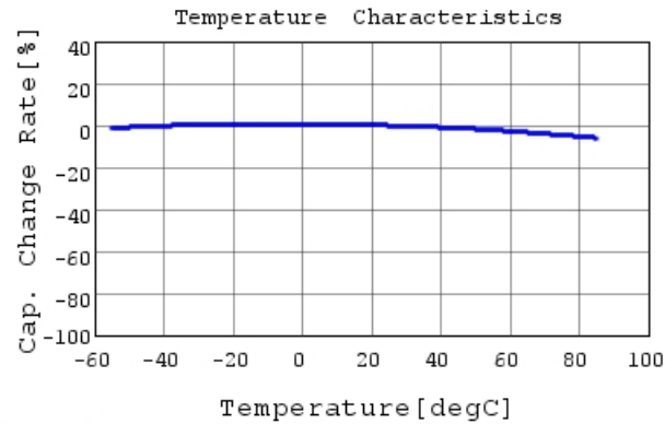
GRM155R61C333KA01 C-Temp. capchange, DC0.0V,
