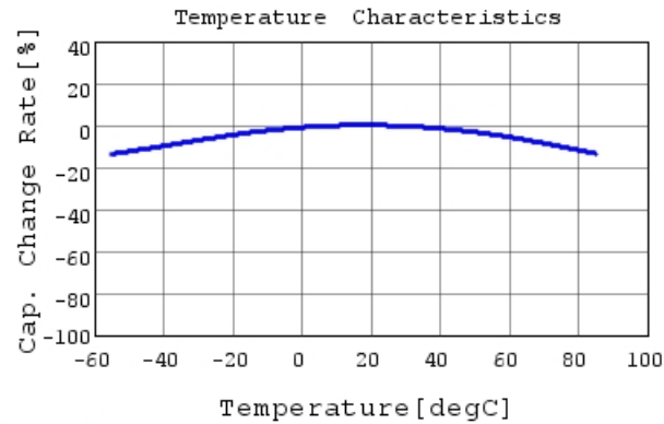
GRM185R61C475KE11 C-Temp. capchange, DC0.0V,
