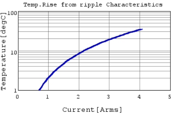
GRM185R61C475KE11 Temp.rise 500kHz
