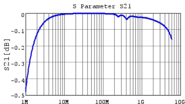
GRM2165C1H472JA01 S21 DCOV, 25degC
