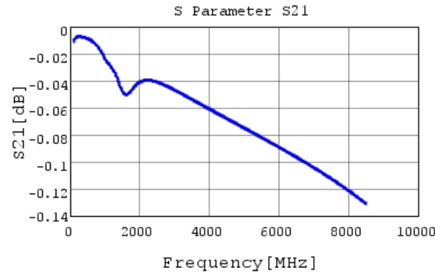
GRT0335C1E471JA02 S21 DCOV, 25degC
