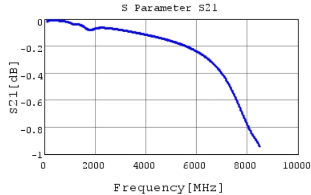
GRT1555C1H271JA02 S21 DCOV, 25degC
