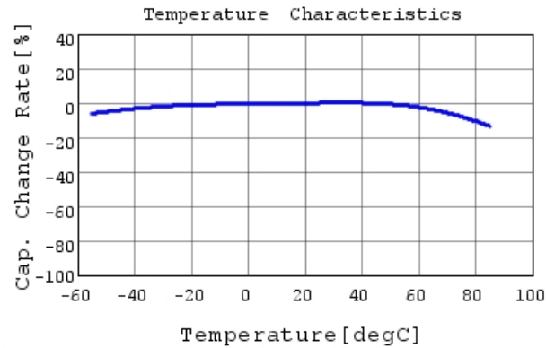
GRT155R60J475ME13 C-Temp. capchange, DC0.0V,
