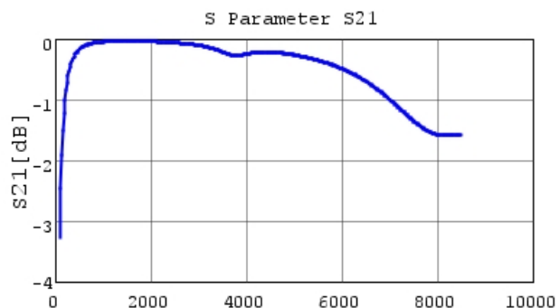
Frequency [MHz] ■ GRT1885C1H150JA02 S21 DCOV, 25degC
