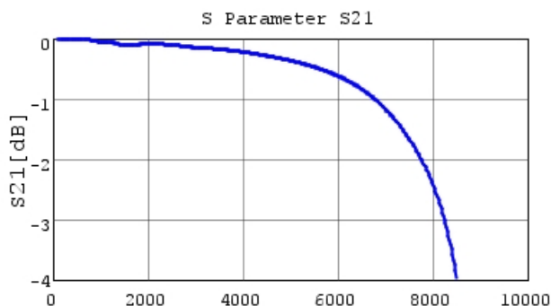
■ GRT1885C1H271JA02 S21 DCOV, 25degC
