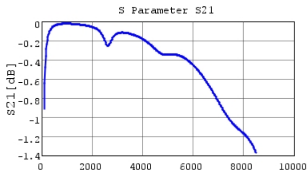
Frequency [MHz] GRT1885C1H330JA02 S21 DCOV, 25degC
